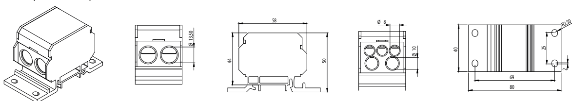
EDBS-50.., EDBS-50../N, EDBS-50../PE
