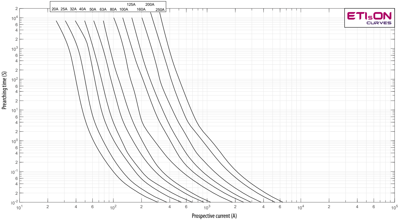
NH2C 500V Time current characteristics I/t, gF
