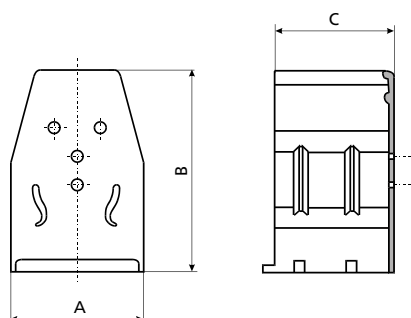
Insulating sleeve of contact spring PK and PP
