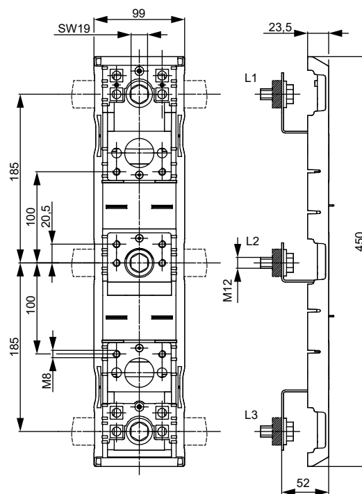
adapter DA 185-100/52
