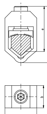
V shaped clamp
