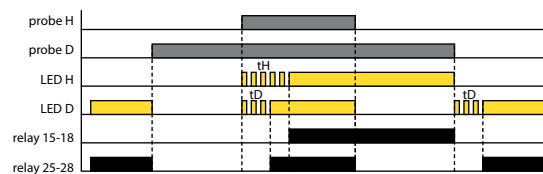
WELL - TANK, ON DELAY (Function 7)
