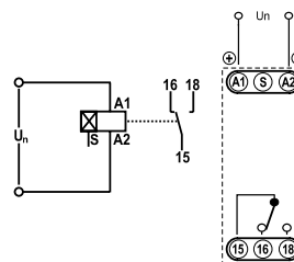
Cycler beginning with pulse
