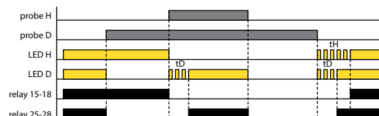
PUMP UP, ON DELAY (Function 5)
