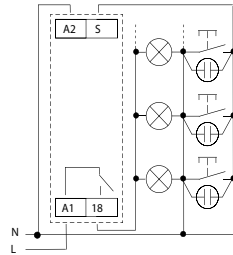
3-wire connection
