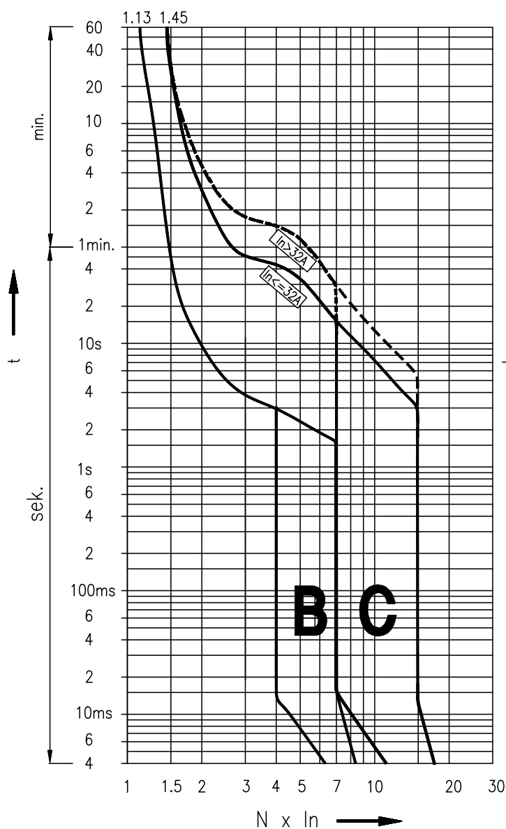
Time current characteristics I/t, ETIMAT P10-DC
