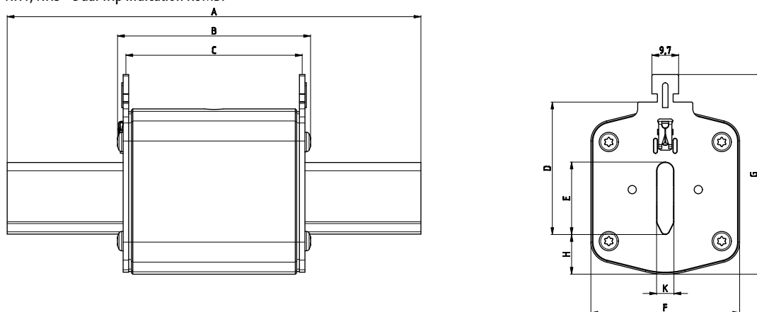
NH1, NH3 - Dual Trip Indication KOMBI
