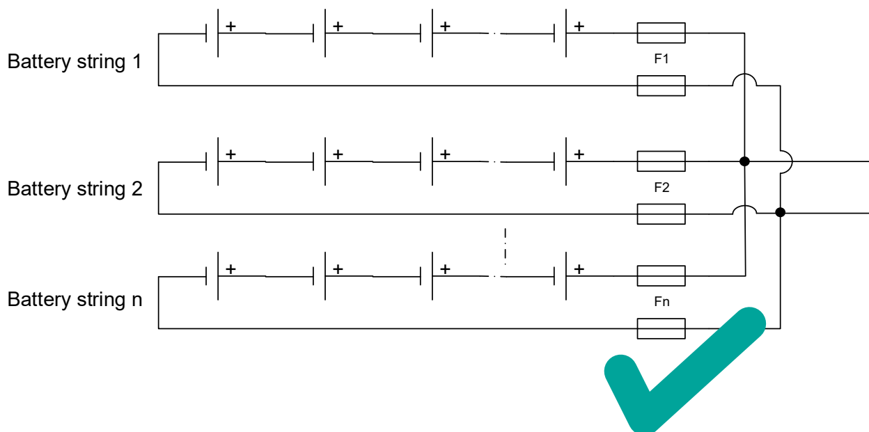
Battery array
