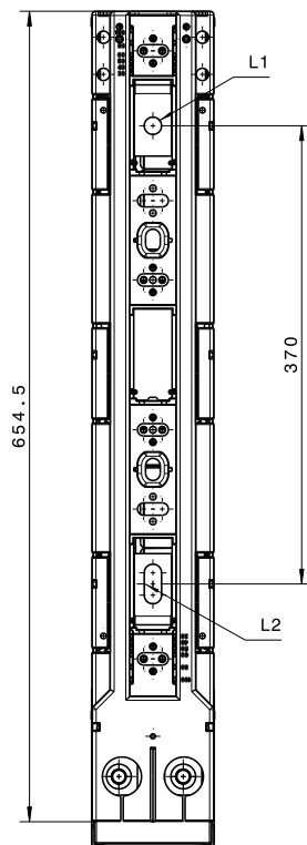
Flat terminal M12
