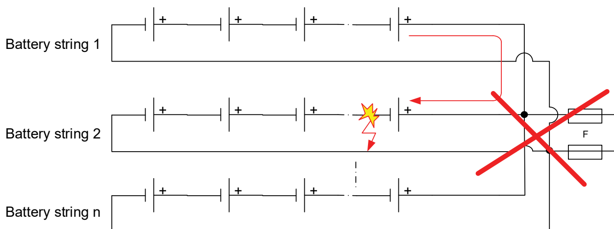
Battery array
