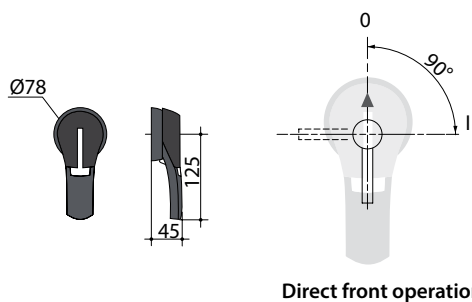
Handle type LBS-EH630
