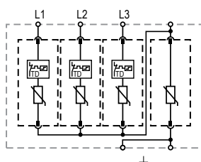
ETITEC M T2 950/20 4Y
