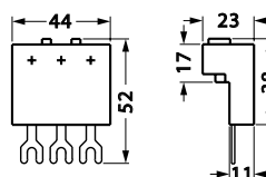
MSP-I22 three-phase head-in terminal, type I
