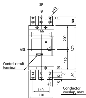
Front connected with Motor Operator
