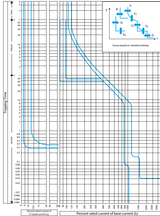
Time/current characteristic curves EB2 630-VE, EB2 800-VE
