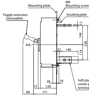
Rear connected
