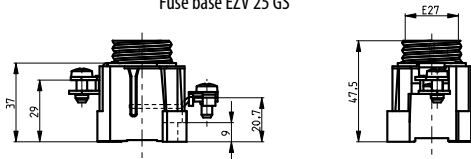
Fuse base EZV 25 GS
