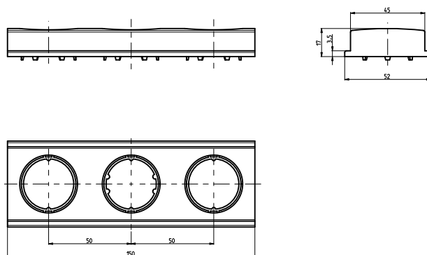
Protective cover GB 63-60
