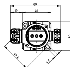
Fuse base EZV 25 GS
