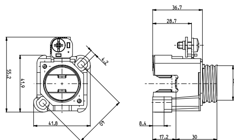
Fuse base EZR 63
