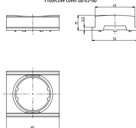
Protective cover GB 63-60
