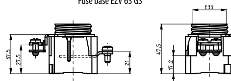
Fuse base EZV 63 GS
