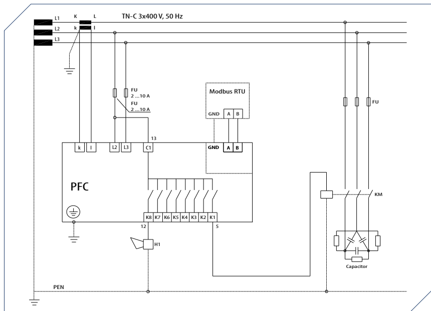
PFC 8 electrical scheme
