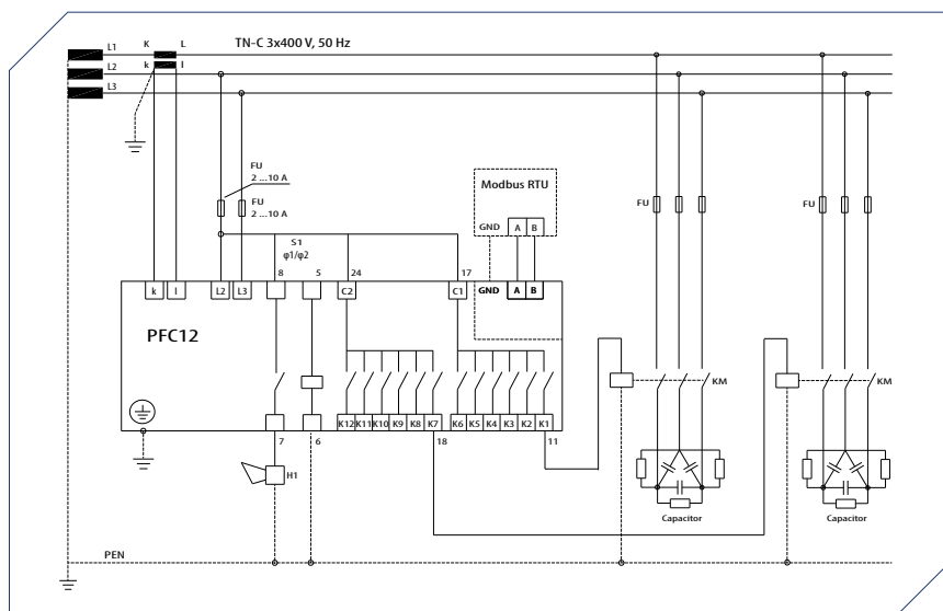
PFC 12 electrical scheme
